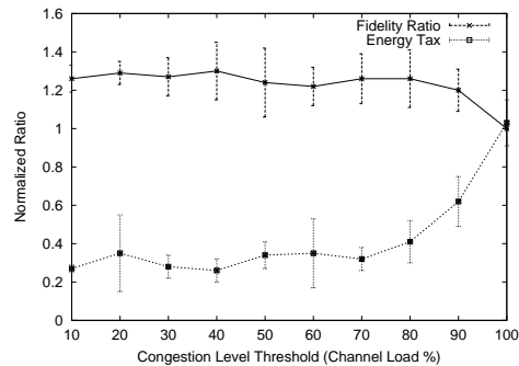
Figure 2: Early Congestion Detection. Different congestion level thresholds that can avoid congestion down the funnel.
