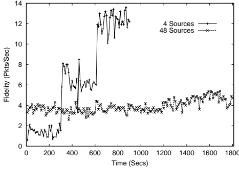
Figure 13: A time series trace showing packet reception rate at the physical sink. The four nodes in the source cluster each send at 5 pkts/sec. When all 48 motes are sources, the rate is \frac{1}{6} pkts/sec. Each trace comprises three intervals corresponding respectively to 0, 1 and 2 VSs activated in the network. Performance gain due to VS participation is immediate but the magnitude depends strongly on traffic pattern and VS placement.
