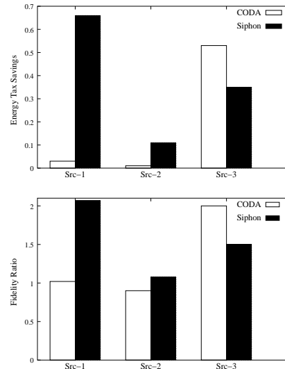
Figure 9: Siphon performance in a real sensor network of 30 nodes. Notice the CODA priority in favor of Src-3.
