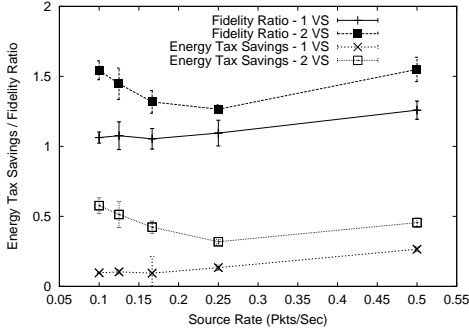
Figure 11: All nodes are Surge sources. Siphon provides increasing performance advantage as the channel load increases in the network. Activating an additional VS boosts this gain. The ‘2 VS’ curves exhibit a routing algorithm artifact at low rates.
