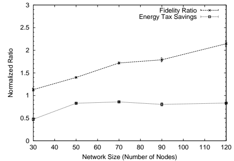
Figure 4: Fidelity and Energy Tax performance in a network with always-on virtual sinks.
