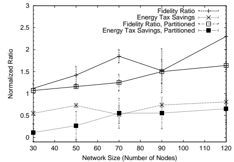
Figure 5: Fidelity and Energy Tax performance in a network where virtual sinks are only activated when congestion is detected, (i.e. on-demand).
