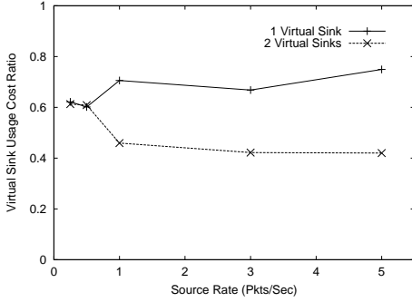
Figure 14: VS Usage Cost Ratio measures the energy cost of using VS to deliver packets to the physical sink normalized by the cost of delivering the same number of packets using only the primary radio network. In terms of the packet transmission costs captured by our energy model, using Siphon actually saves energy.
