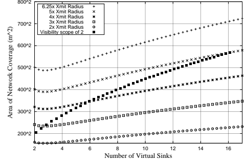
Figure 7: Requirement for a connected secondary network. The transmission range of the long-range radio is expressed as multiples of the transmission radius of the low-power radio. The visibility scope requirement that assure both energy tax and fidelity improvements is plotted as filled square in the figure.
