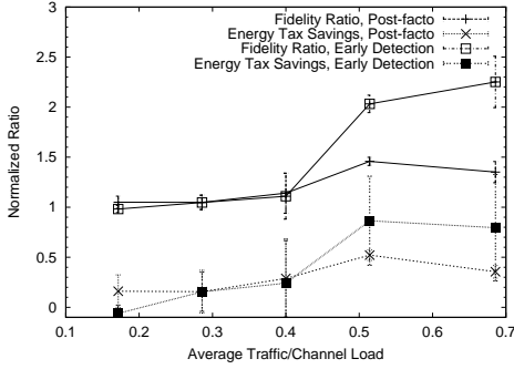
Figure 10: Post-facto traffic redirection versus the early-detection approach.
