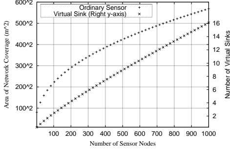
Figure 6: Number of sensor nodes required to ensure connectivity in the corresponding areas of network coverage as well as the number of virtual sinks (right vertical axis) required to ensure performance improvements.
