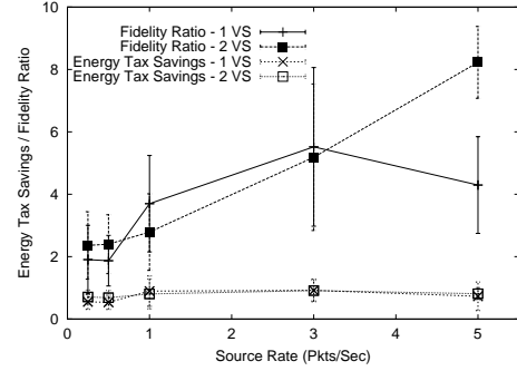
Figure 12: A cluster of 4 nodes are Surge sources. Siphon provides increasing performance advantage as channel load increases in the network. Activating an additional VS has little effect due to VS placement and packet propagation patterns.
