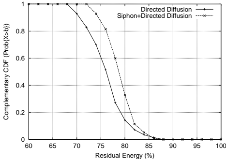
Figure 8: Energy Distribution (CDF) of a 70-node network with 3 virtual sinks scattered randomly across the network. With Siphon’s load balancing feature more nodes share the energy load. Therefore, fewer nodes have residual energy larger than 85%, but more nodes have larger residual energy (e.g., the percentage of nodes having residual energy larger than 75% increases from 60% to 85%), effectively increasing the lifetime of the network.
