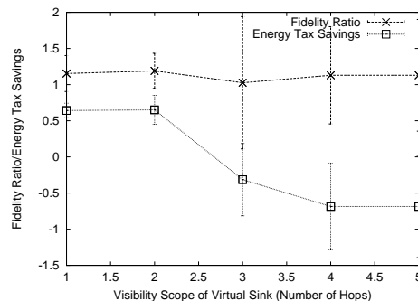
Figure 3: The impact of the visibility scope of a VS for a network of 30 nodes.
